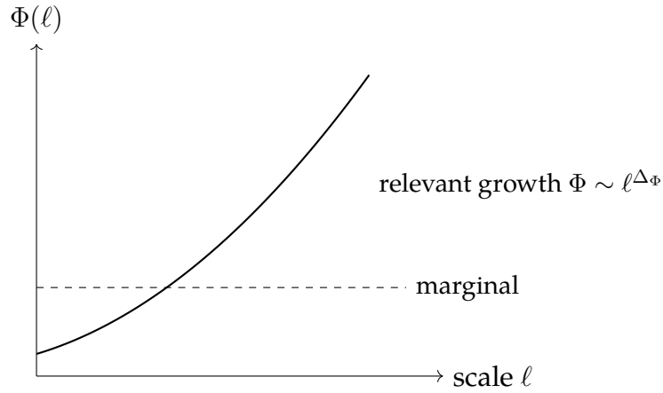
Figure 18: Visibility as a relevant operator: \Phi(\ell) grows under scale transformation while a marginal operator would remain constant. The superlinear growth drives entropy production and instability at large scales.
