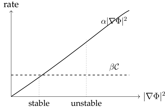
Figure 5: Entropy production \alpha|\nabla\Phi|^2 grows without bound while corrective capacity \beta\mathcal{C} is bounded. Instability begins where the curves cross.
